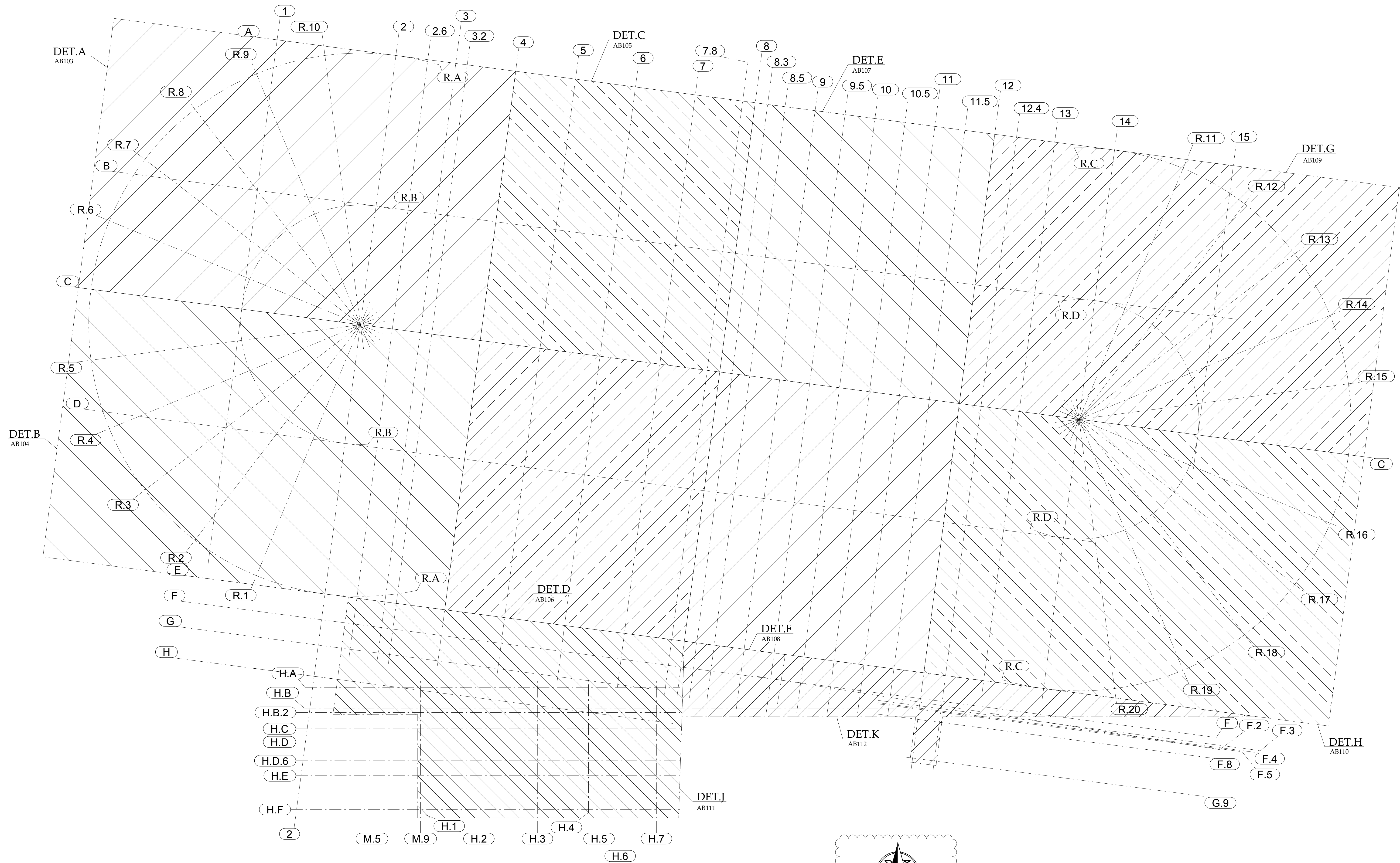
ANCHOR BOLT KEY PLAN (REF. SHEET: S1100)
