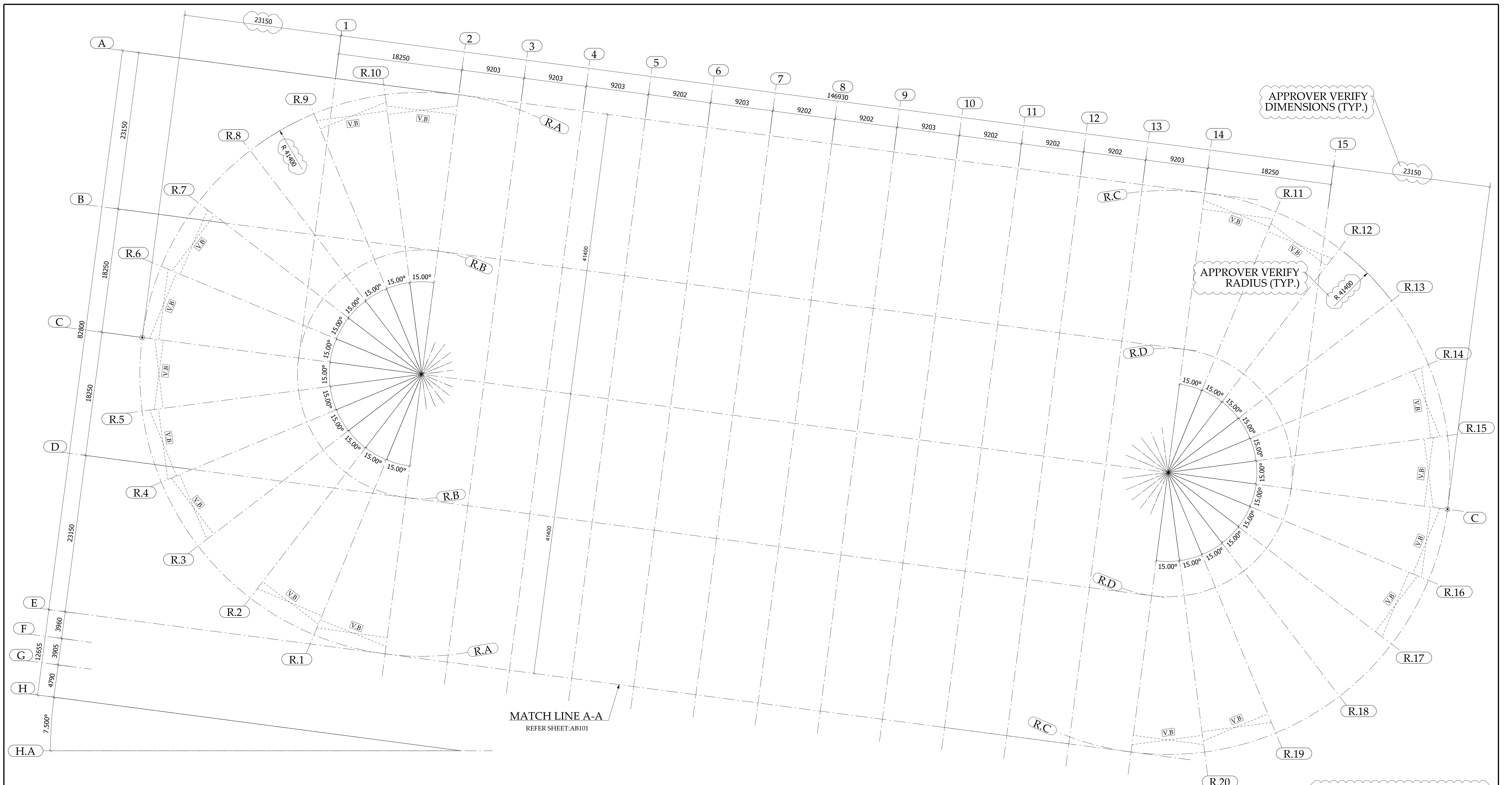
PARTIAL GRID LAYOUT PLAN AREA 'A' & 'B' (REF. SHEET: S1100)
