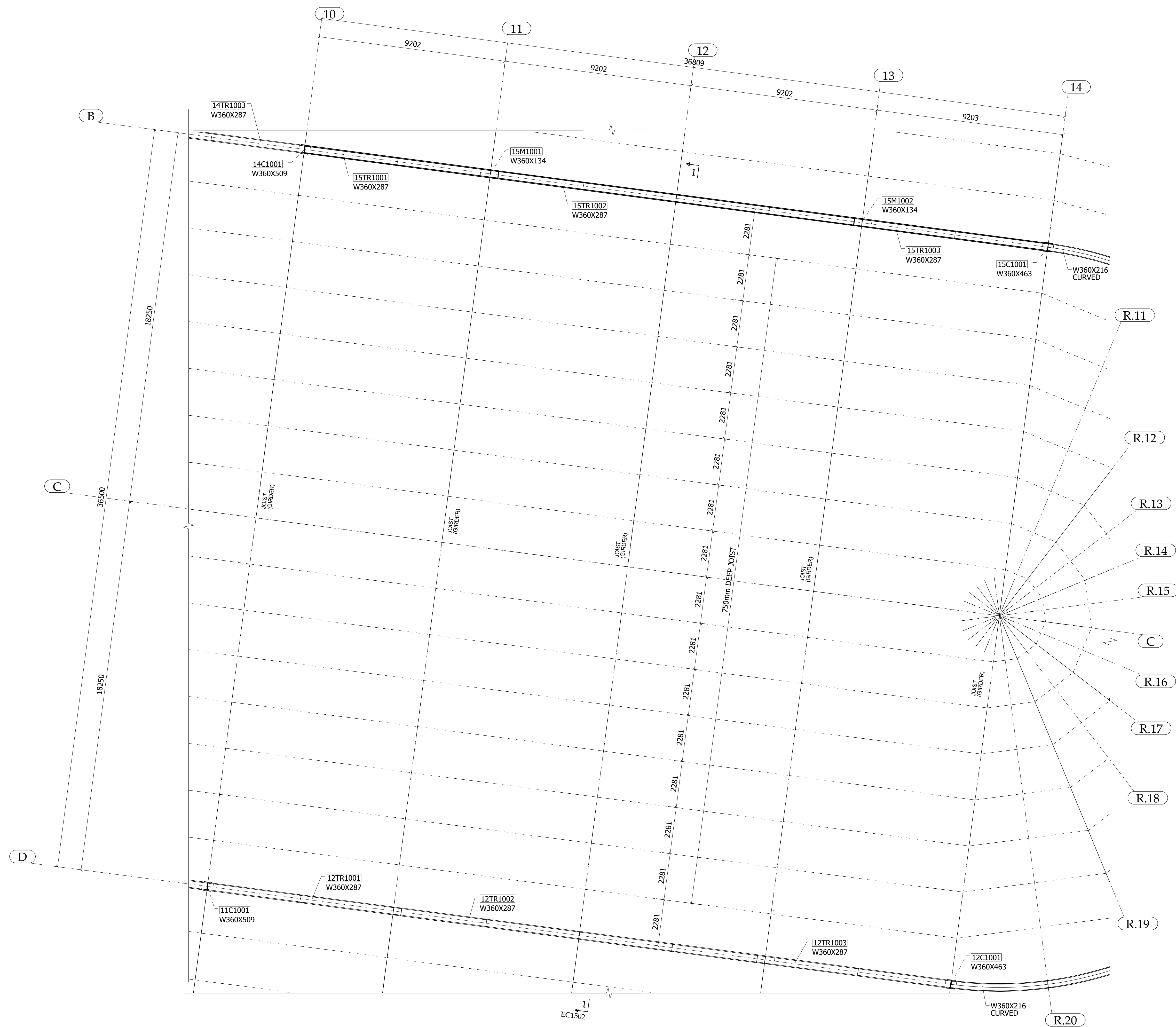
ROOF FRAMING PLAN (PHASE-15) (SECTOR A&B) (REF. SHEET: S1420)
