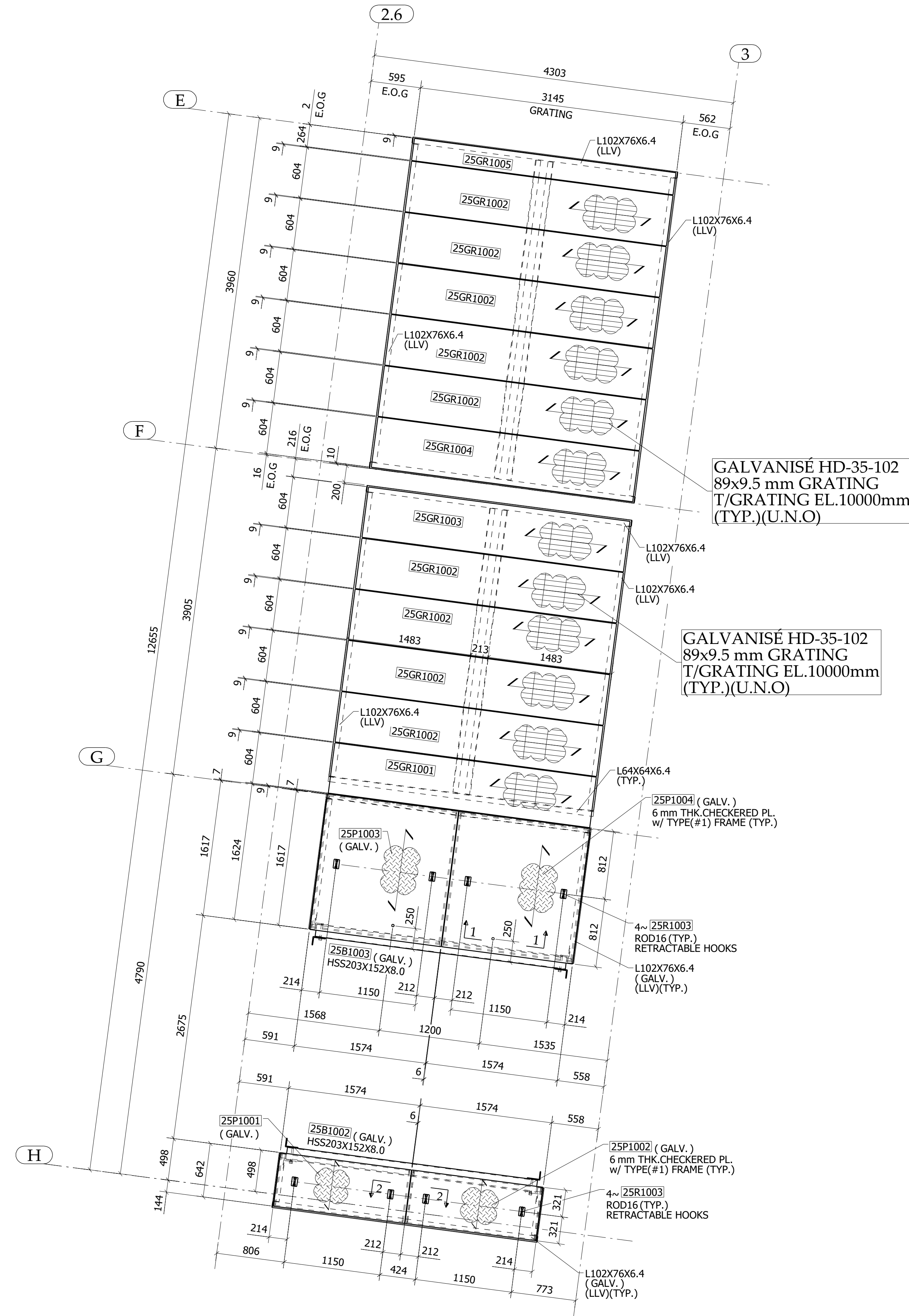
SNOW PIT SUPPORT GRATING FRAMING PLAN (SECTOR C) T/GRATING EL.10000mm TYP. (U.N.O.) (REF. SHEET: 5003A/5003)
