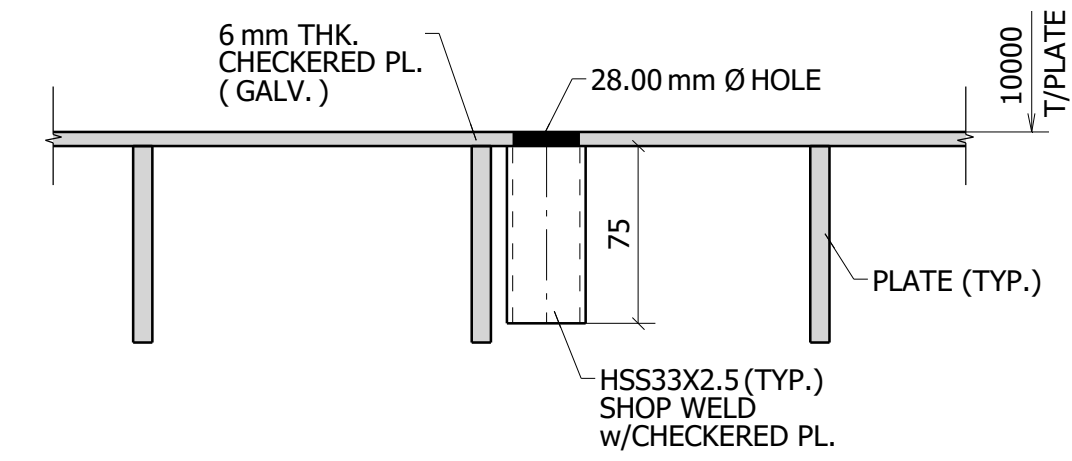
SECTION 1 - 1 TUBULAR TUBE TYPICAL DETAIL (REF. SEC: 5003P/5003)
