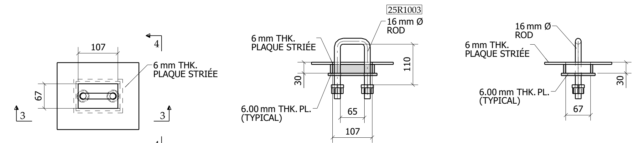
SECTION 3 - 3 RETRACTABLE HOOK DETAIL (REF. SEC: 5003Q/5003)
