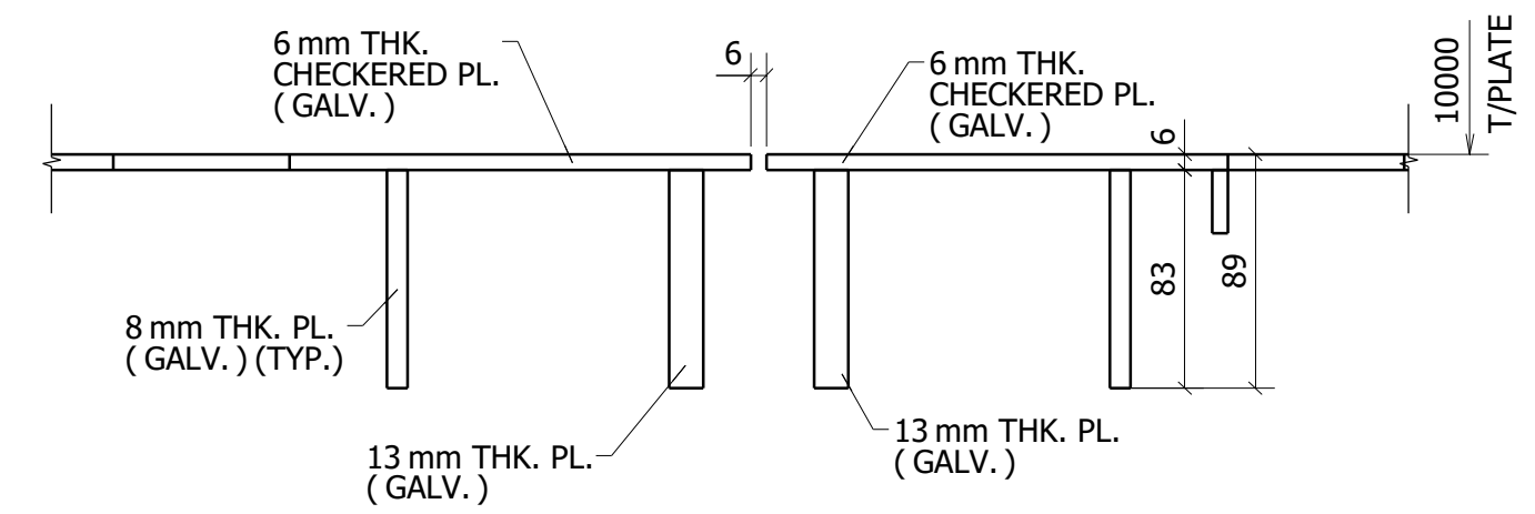
SECTION 2 - 2 TYPICAL PLATE ARRANGEMENT DETAIL (REF. SEC: 5003D/5003)
